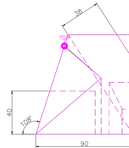
RIGHT SCALE 1/2
