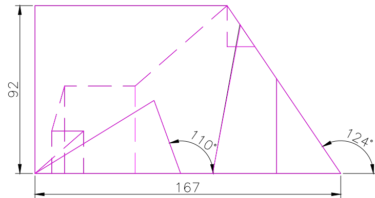
FRONT SCALE 1/2
