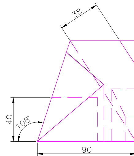
RIGHT SCALE 1/2
