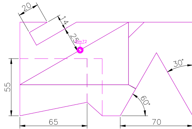
TOP SCALE 1/2
