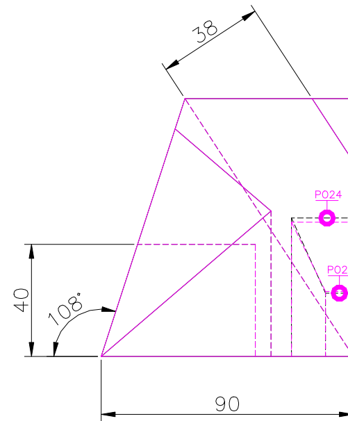
RIGHT SCALE 1/2
