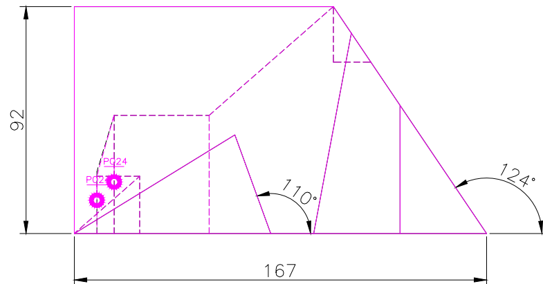
FRONT SCALE 1/2
