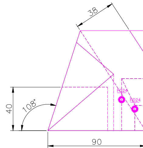
RIGHT SCALE 1/2
