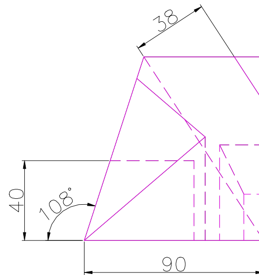
RIGHT SCALE 1/2
