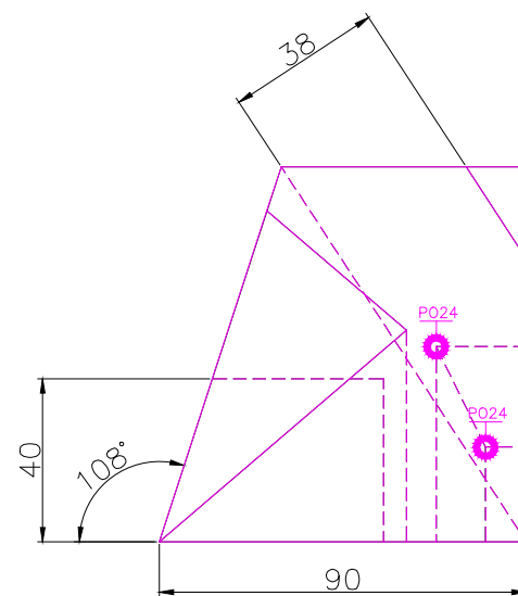
RIGHT SCALE 1/2
