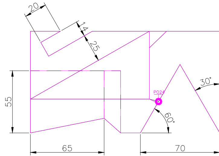
TOP SCALE 1/2
