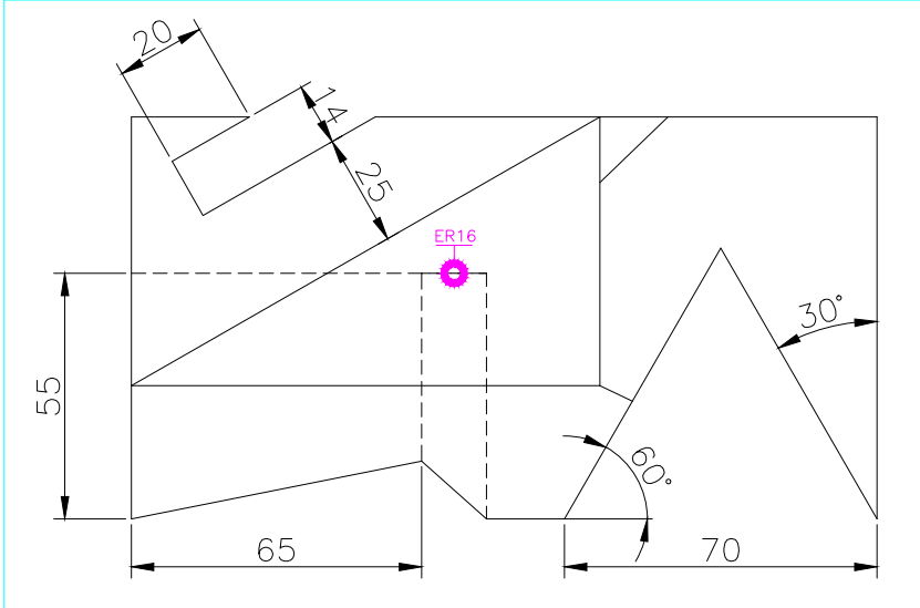
TOP SCALE 1/2
