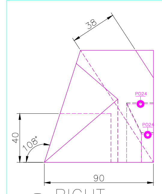
RIGHT SCALE 1/2
