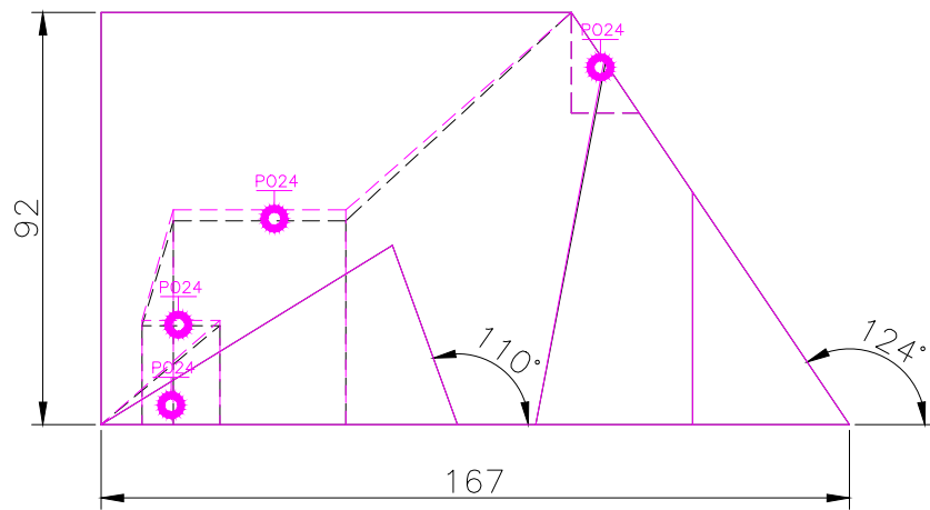
FRONT SCALE 1/2
