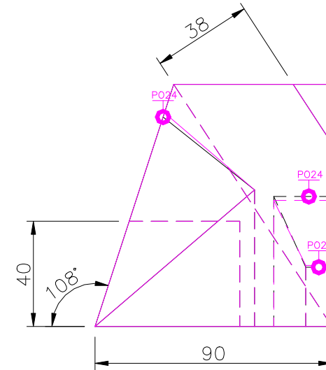
RIGHT SCALE 1/2
