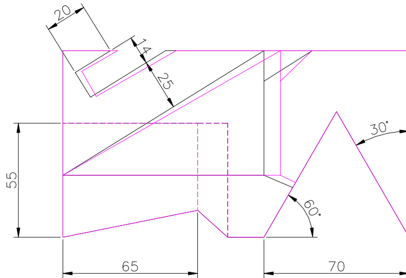
TOP SCALE 1/2
