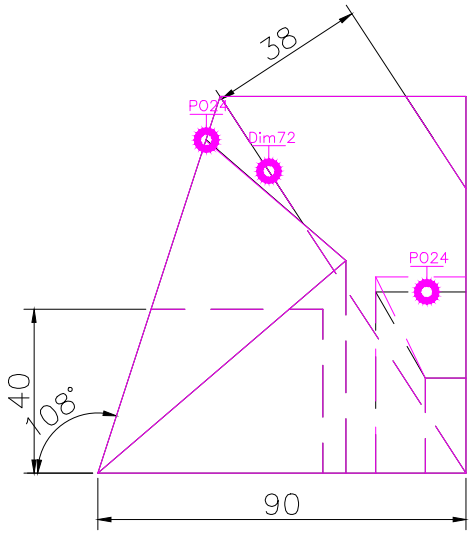
RIGHT SCALE 1/2
