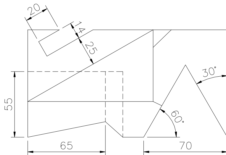
TOP SCALE 1/2
