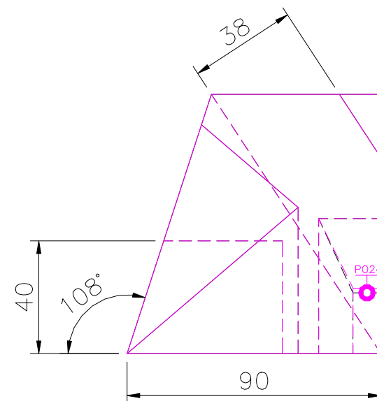
RIGHT SCALE 1/2
