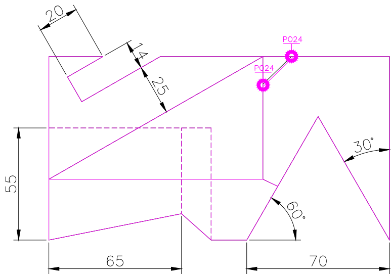
TOP SCALE 1/2
