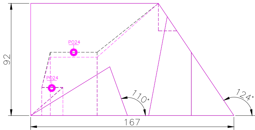
FRONT SCALE 1/2
