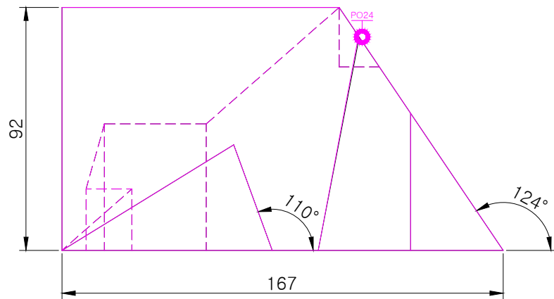
FRONT SCALE 1/2
