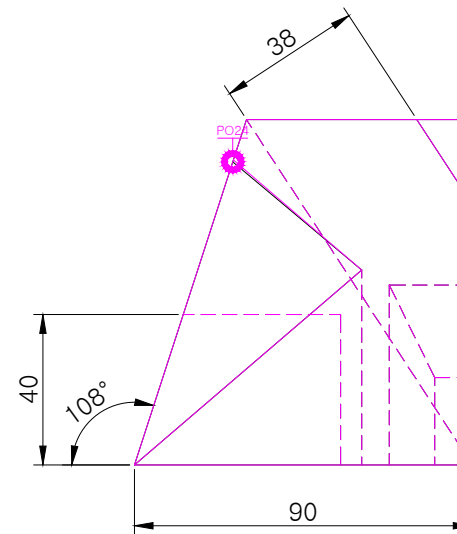
RIGHT SCALE 1/2
