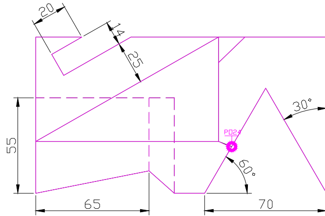
TOP SCALE 1/2
