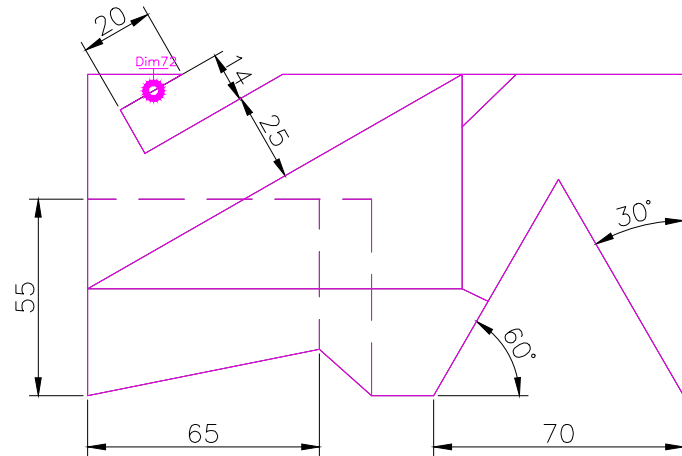
TOP SCALE 1/2
