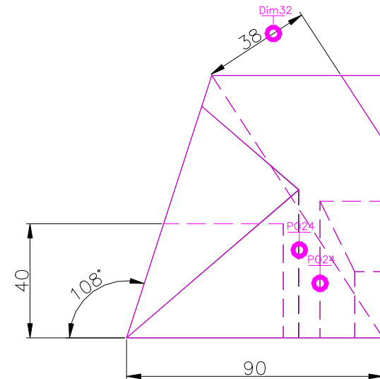
RIGHT SCALE 1/2
