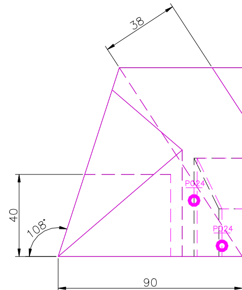
RIGHT SCALE 1/2
