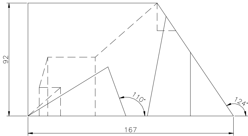
FRONT SCALE 1/2
