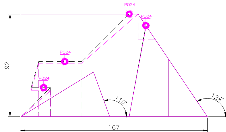
FRONT SCALE 1/2
