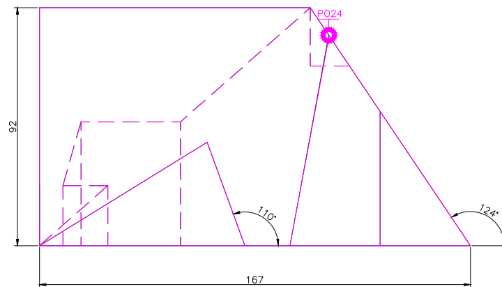
FRONT SCALE 1/2
