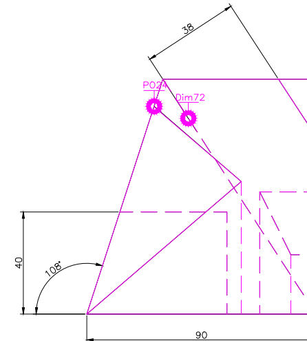
RIGHT SCALE 1/2
