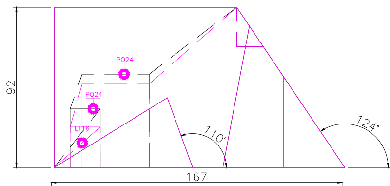
FRONT scale 1/2
