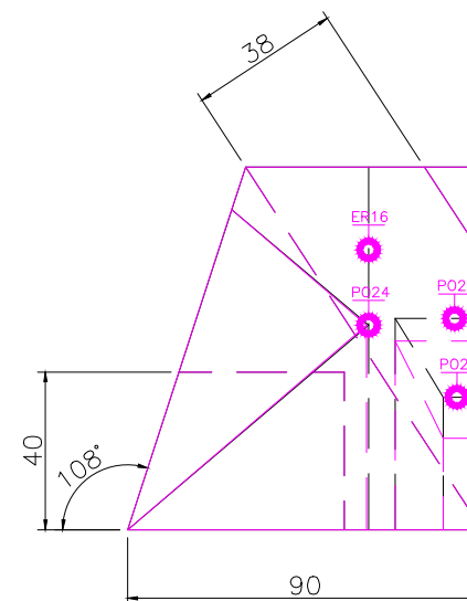
RIGHT scale 1/2
