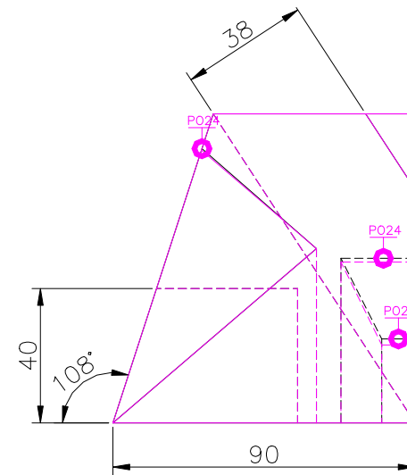
RIGHT SCALE 1/2
