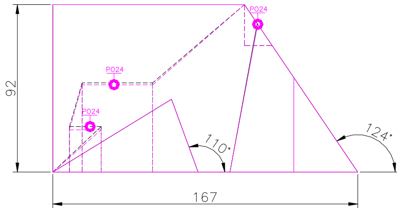
FRONT SCALE 1/2
