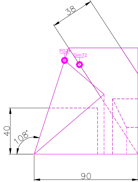
RIGHT SCALE 1/2
