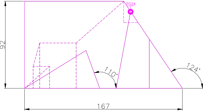
FRONT SCALE 1/2
