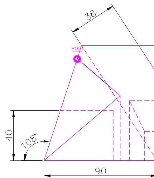
RIGHT SCALE 1/2
