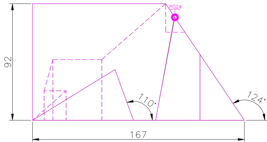
FRONT SCALE 1/2
