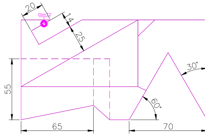
TOP SCALE 1/2
