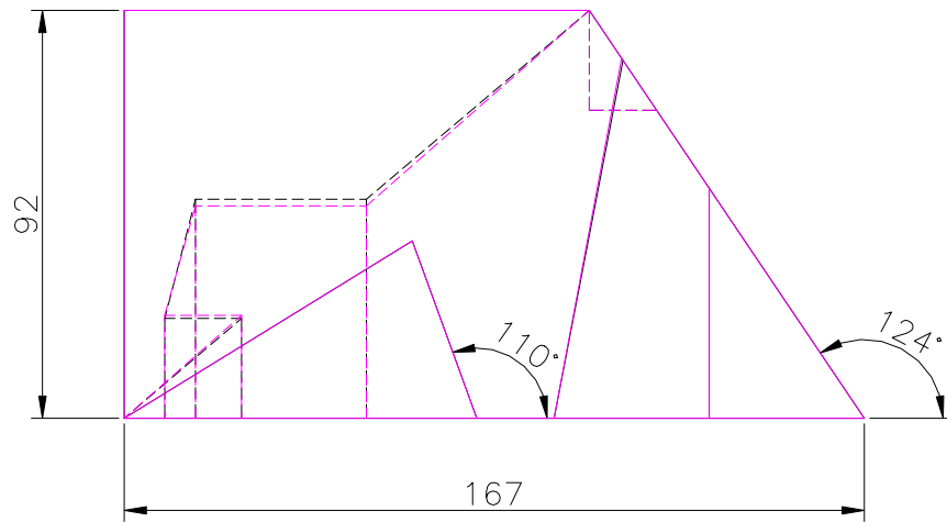
FRONT SCALE 1/2
