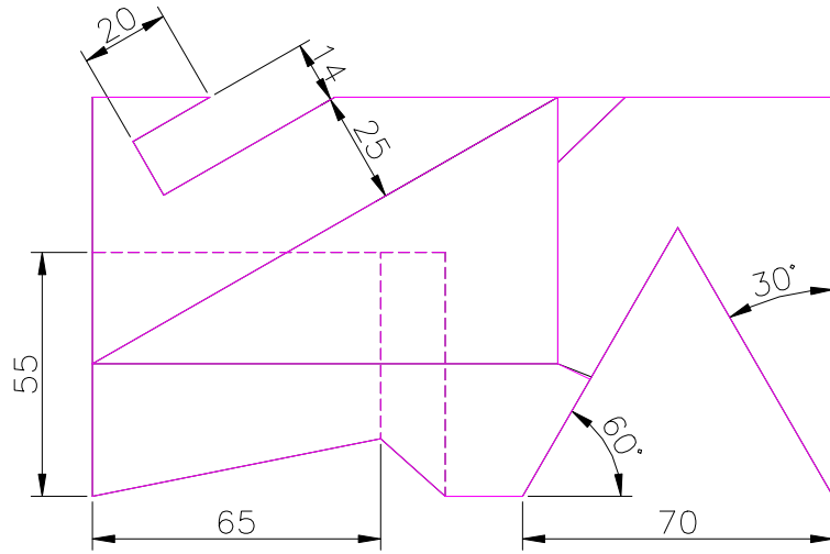
TOP SCALE 1/2
