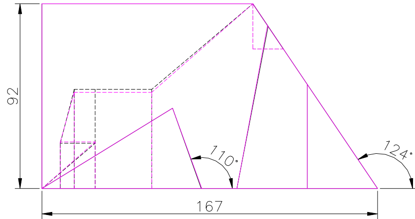
FRONT SCALE 1/2
