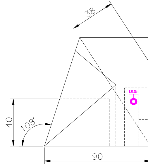
RIGHT SCALE 1/2
