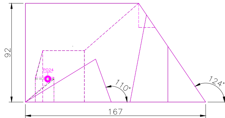
FRONT SCALE 1/2
