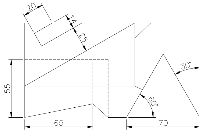
TOP SCALE 1/2
