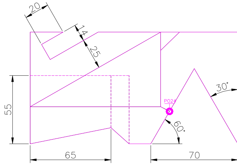
TOP SCALE 1/2
