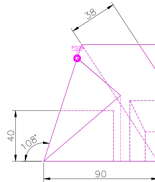
RIGHT SCALE 1/2
