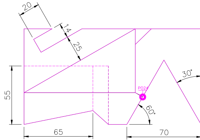
TOP SCALE 1/2
