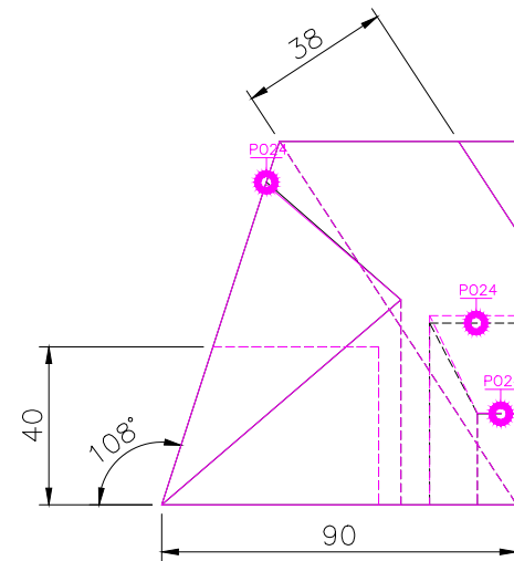
RIGHT SCALE 1/2
