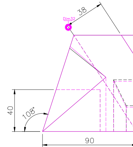
RIGHT SCALE 1/2
