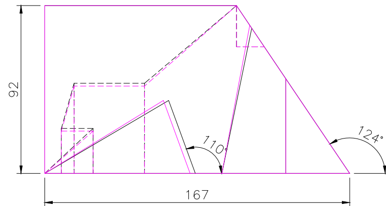
FRONT SCALE 1/2
