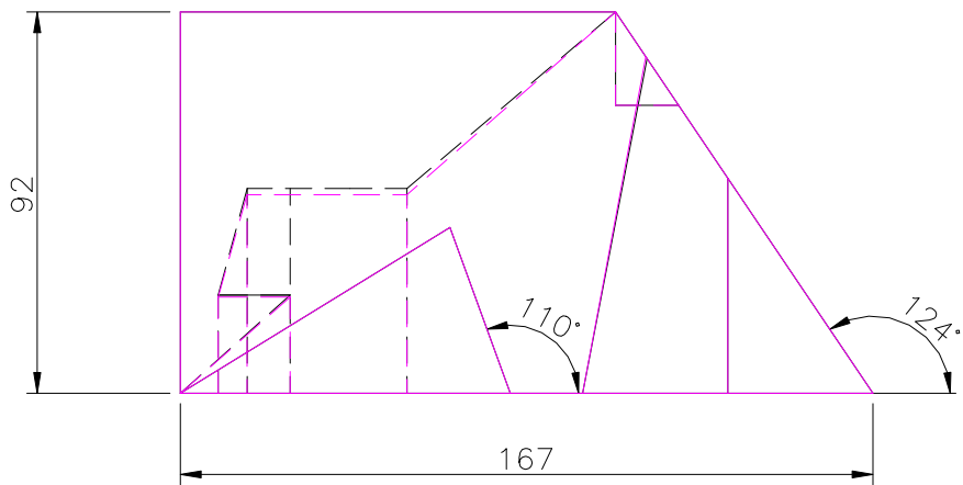
FRONT SCALE 1/2
