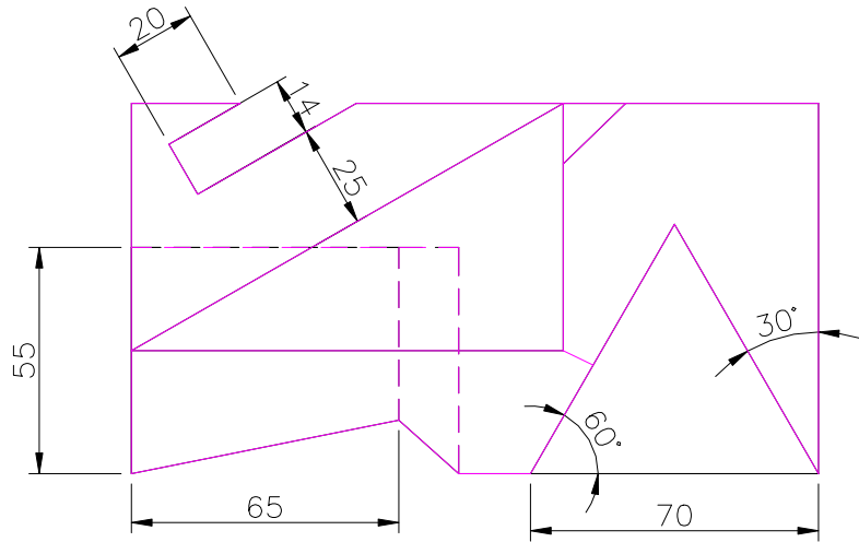
TOP SCALE 1/2
