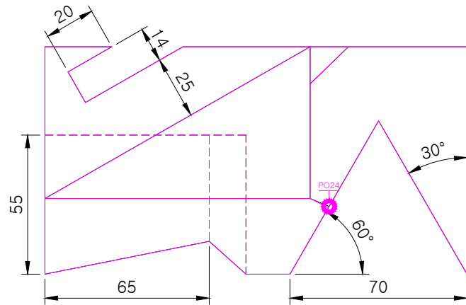
TOP SCALE 1/2
