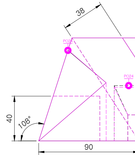
RIGHT SCALE 1/2
