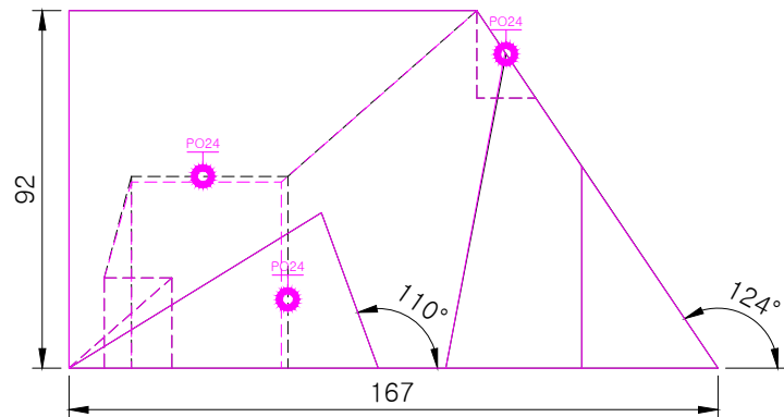
FRONT SCALE 1/2
