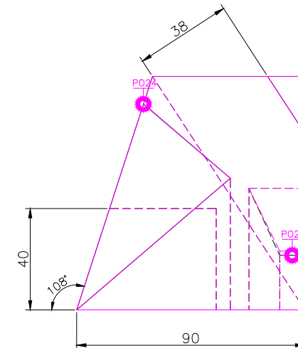
RIGHT SCALE 1/2
