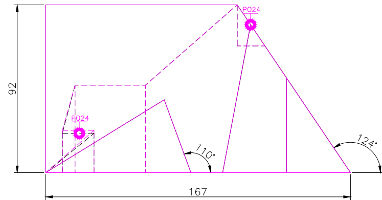
FRONT SCALE 1/2
