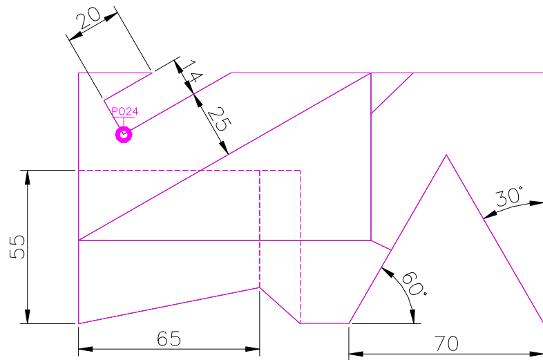
TOP SCALE 1/2
