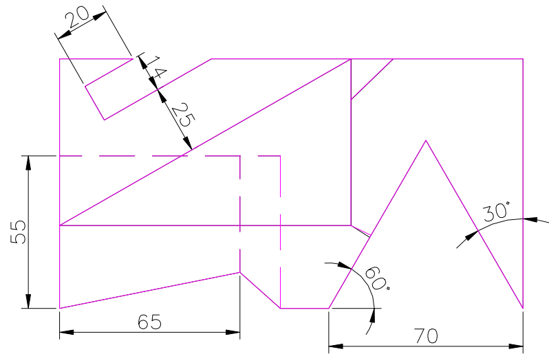
TOP SCALE 1/2
