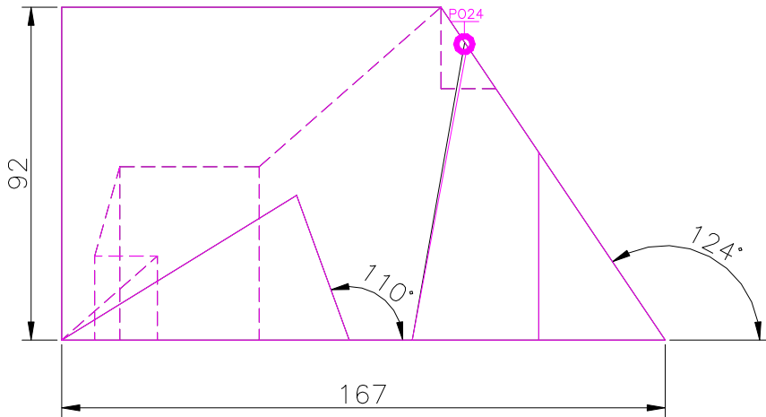
FRONT SCALE 1/2
