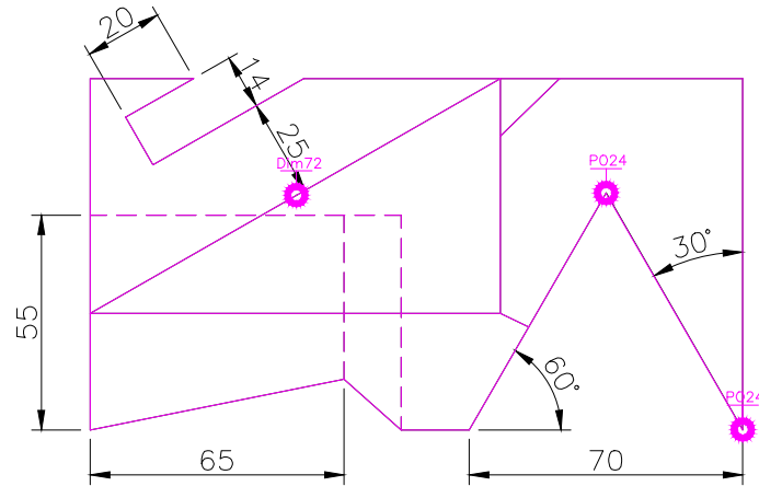
TOP SCALE 1/2
