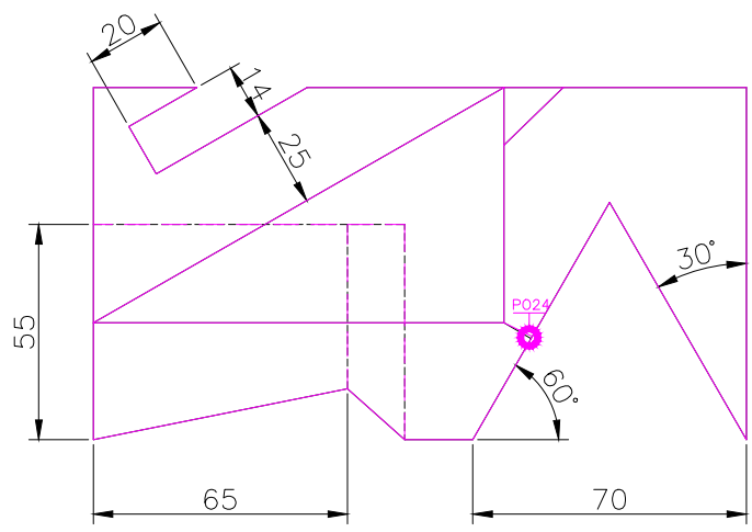
TOP SCALE 1/2
