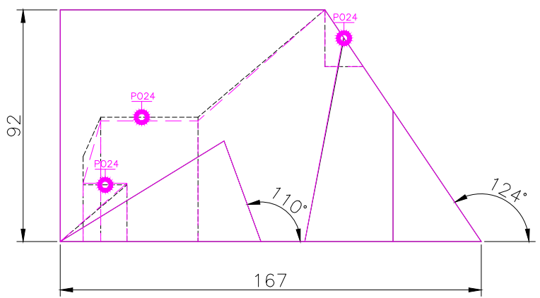
FRONT SCALE 1/2
