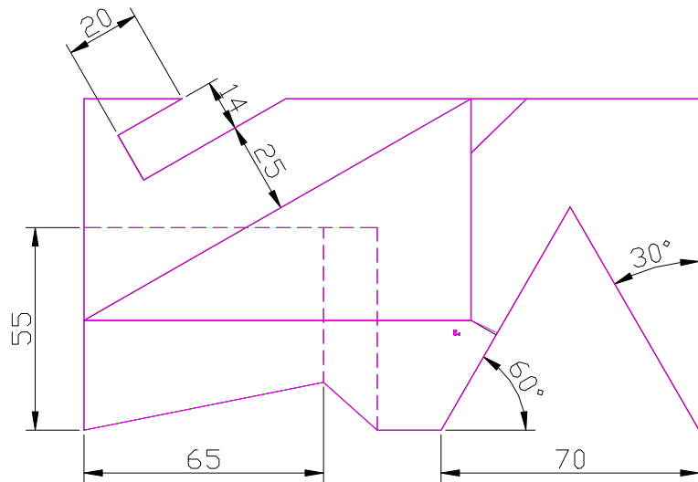
TOP SCALE 1/2
