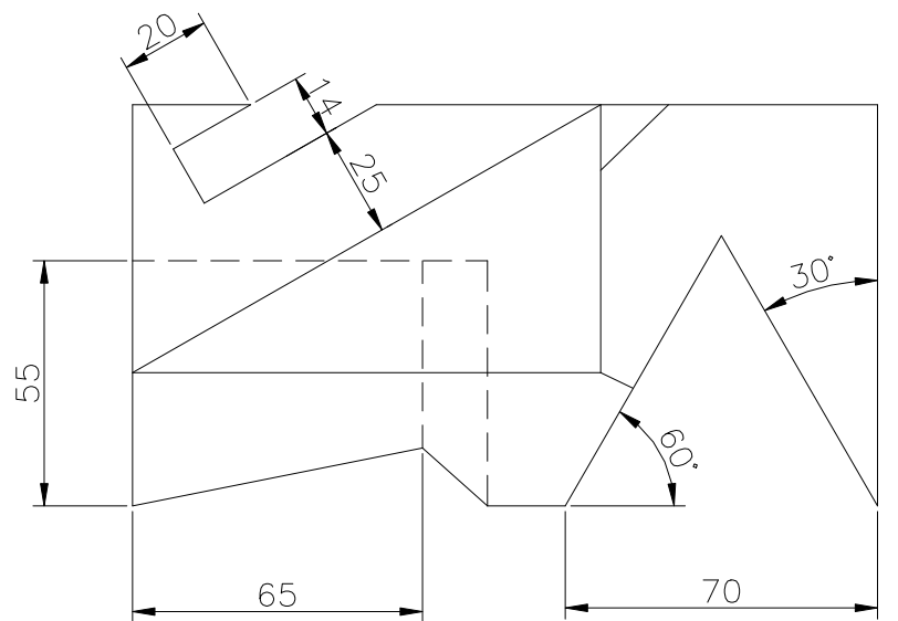
TOP SCALE 1/2
