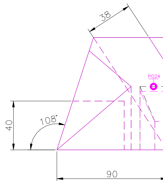
RIGHT SCALE 1/2
