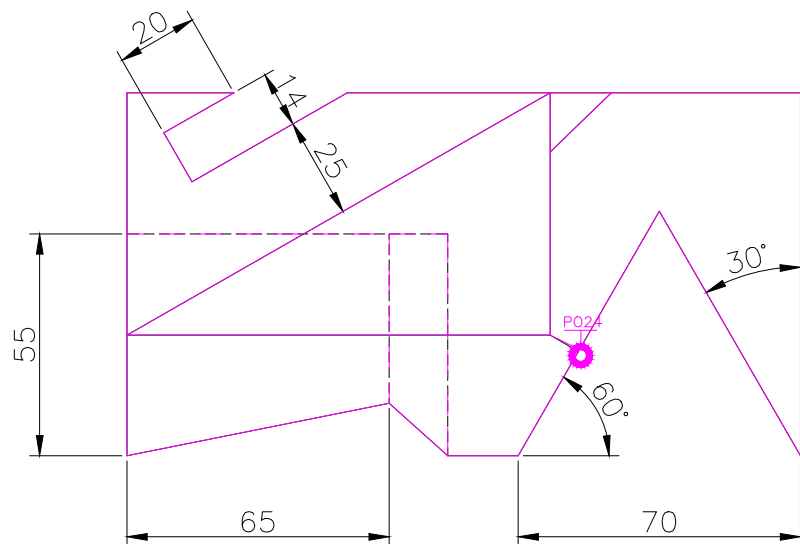
TOP SCALE 1/2
