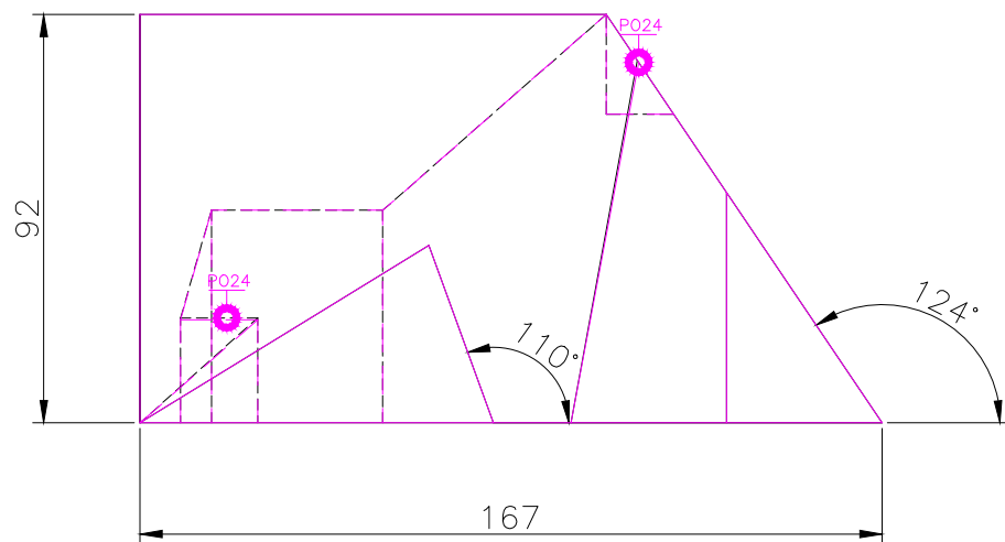
FRONT SCALE 1/2
