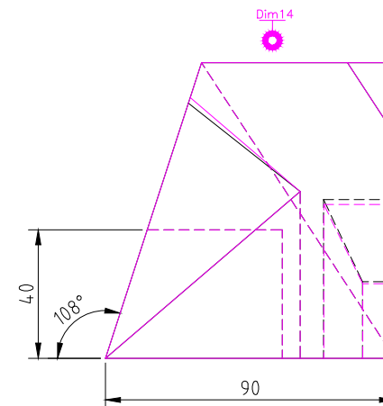
RIGHT SCALE 1/2
