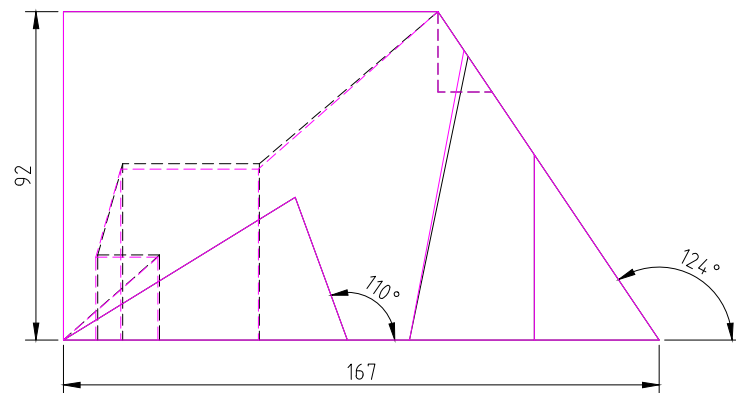
FRONT SCALE 1/2
