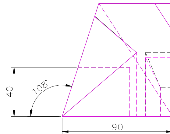
RIGHT SCALE 1/2
