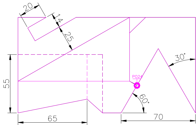
TOP SCALE 1/2
