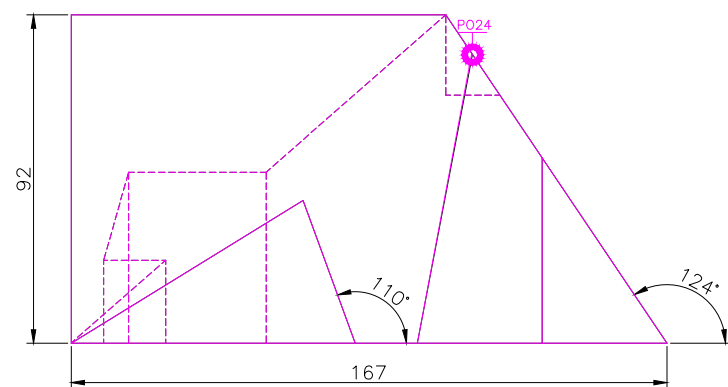
FRONT SCALE 1/2
