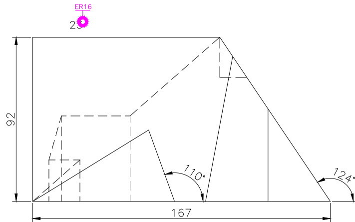
FRONT SCALE 1/2
