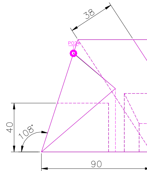
RIGHT SCALE 1/2
