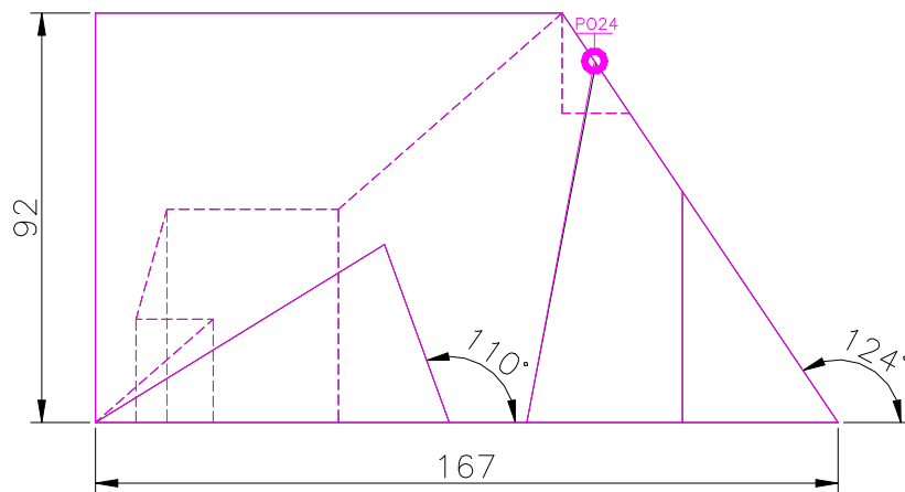
FRONT SCALE 1/2
