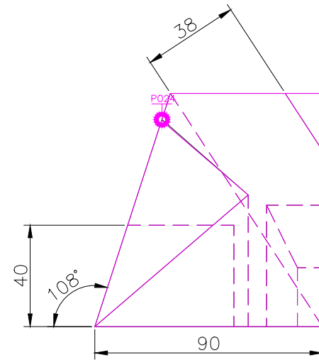
RIGHT SCALE 1/2
