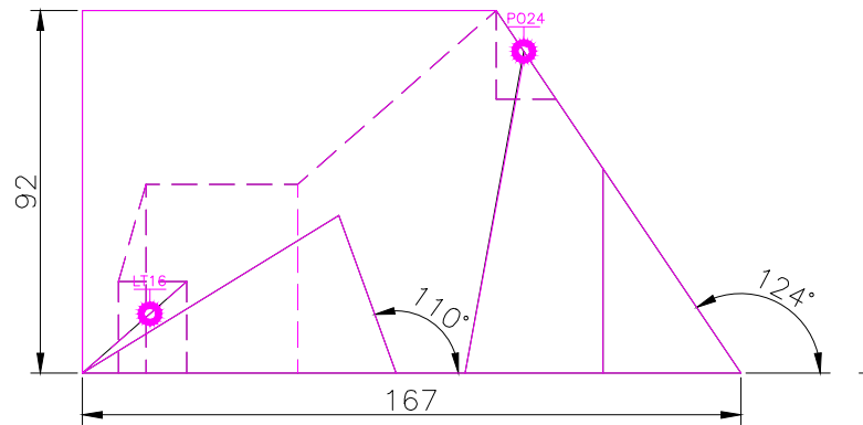
FRONT SCALE 1/2
