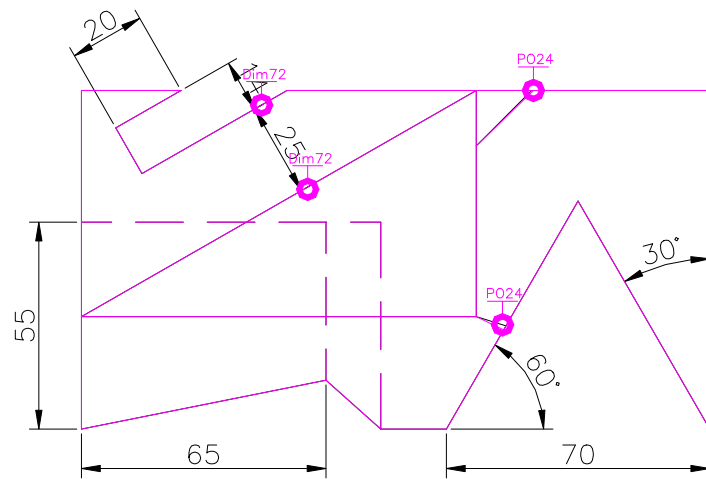
TOP SCALE 1/2
