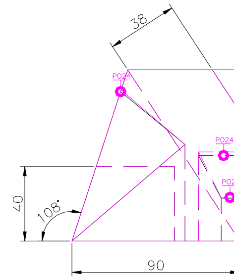
RIGHT SCALE 1/2
